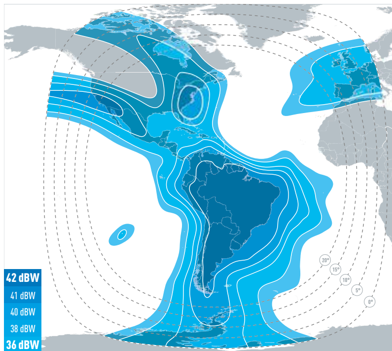
C-BAND DOWNLINK COVERAGE
