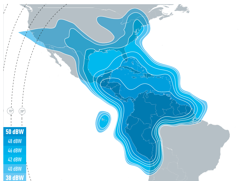
KU-BAND AMERICAS DOWNLINK COVERAGE
