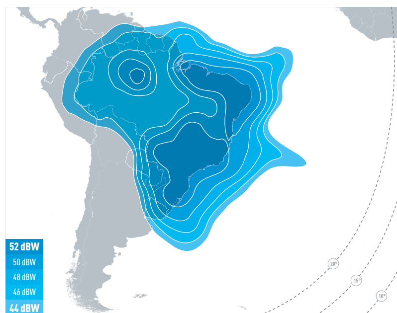
KU-BAND BRAZIL DOWNLINK COVERAGE
